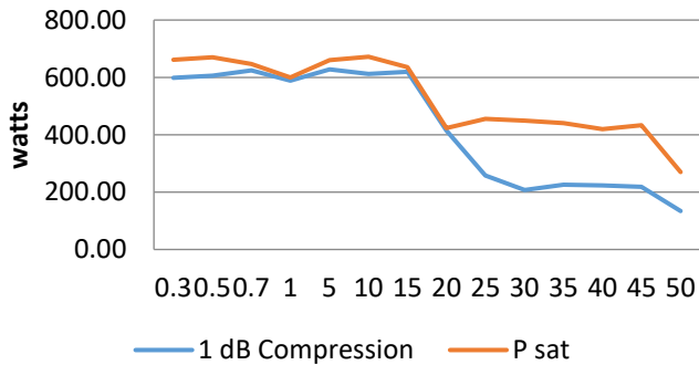
Power v Frequency (MHz)
